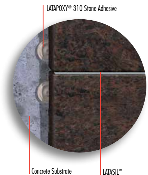
Properly Prepared Concrete, Backer Board or Masonry Substrates (if substrate requires leveling, use 3701 Fortified Mortar Bed)
